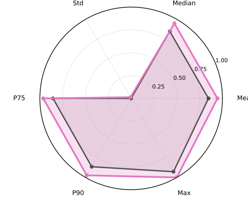
SynthID
