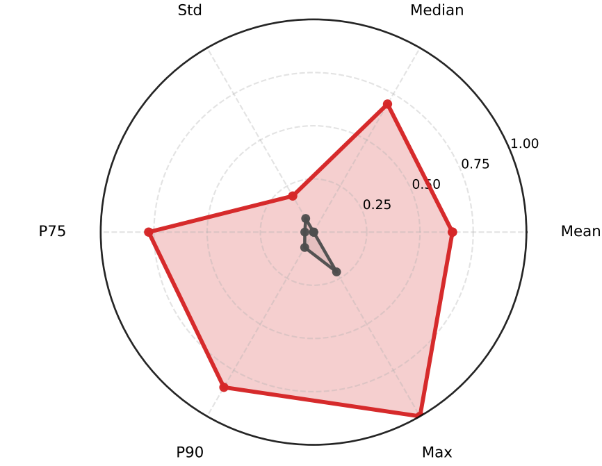
EWD
