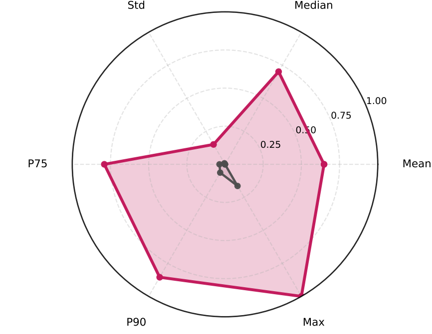
DBSF
