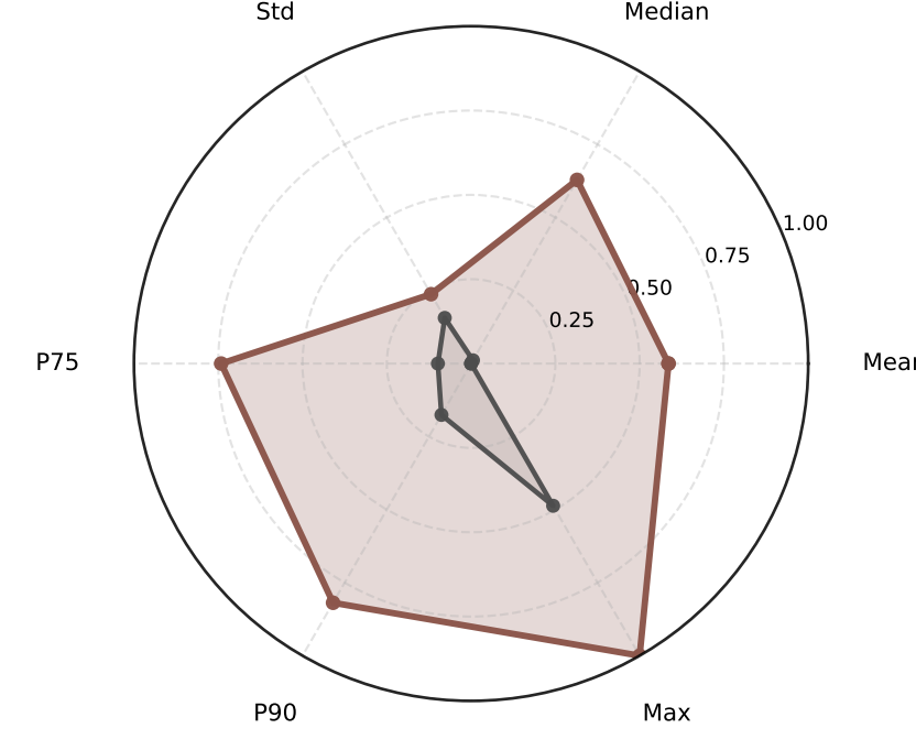
Unbiased
