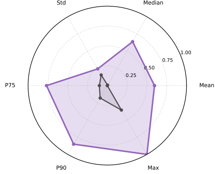
DIP
